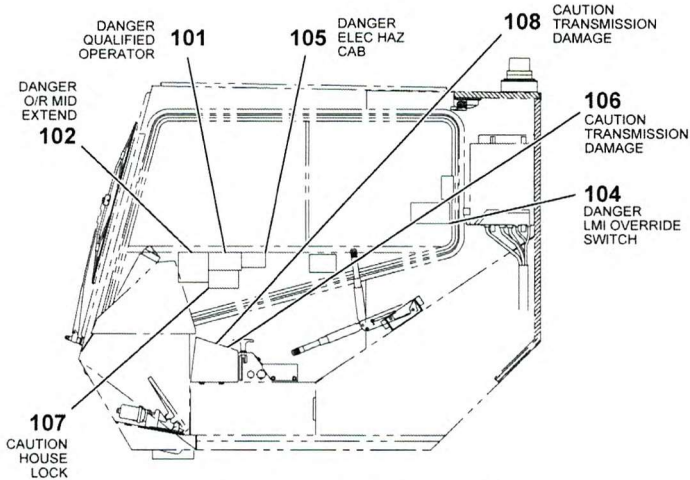
CAB - PARTIAL INSIDE VIEW
