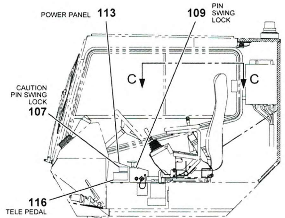
CAB - INSIDE VIEW
