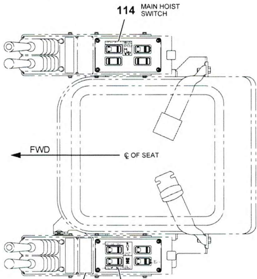
VIEW C-C SEAT
